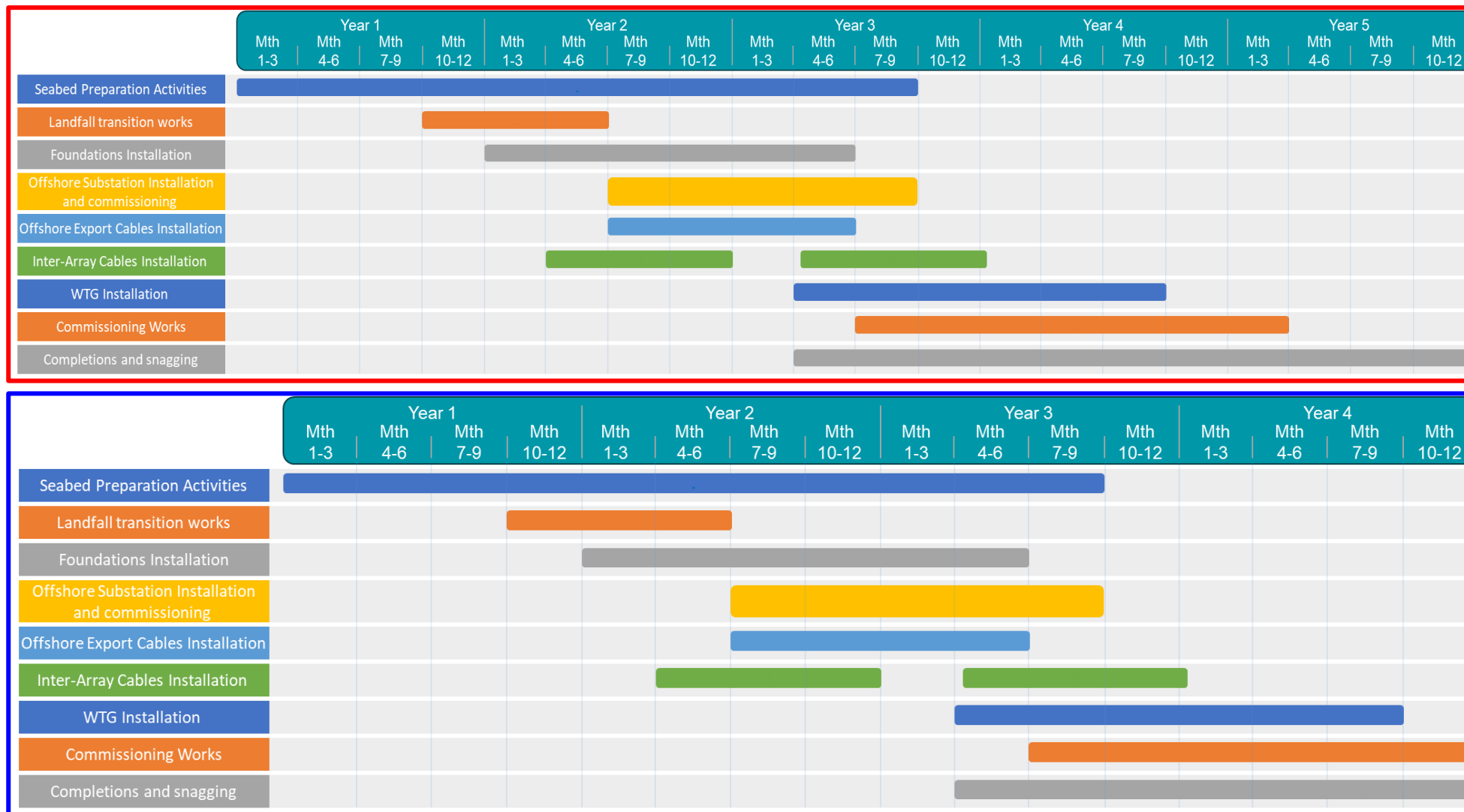
Figure 2.23: High-level construction programme
